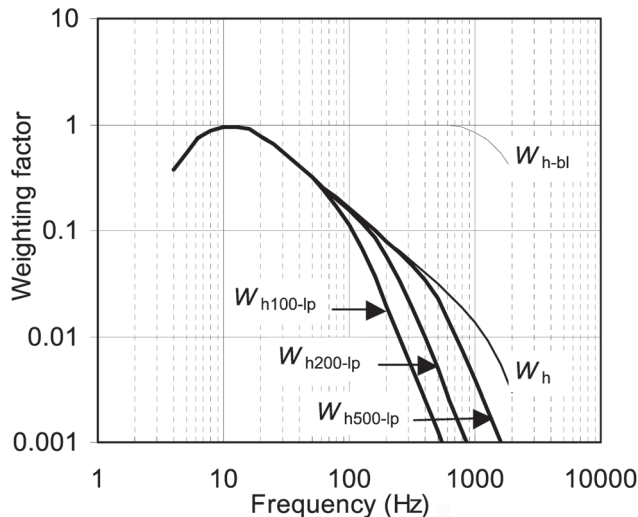
Fig. 3. Comparison of weightings W_h and W_{h-bl} , from ISO 8041 and weightings W_{h100-lp} , W_{h200-lp} and W_{h500-lp} .
